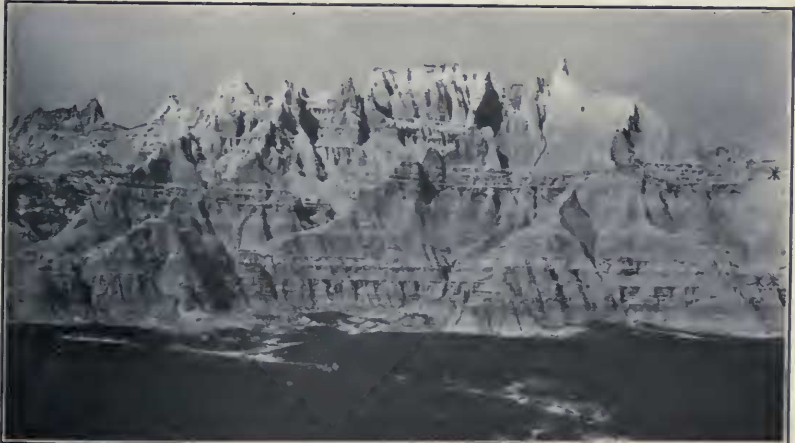
FIG. 2. Section of the Oreodon beds in the Wall of the Badlands at Cedar Pass, north of Interior, Jackson County. The central highest pinnacles are capped by Leptauchenia volcanic ash beds. The subdivision of the Oreodon beds here into upper clays, upper nodular layer, middle clays, and lower nodular layer are clearly shown, especially in the right half of the picture. The upper nodular layer is marked (*) and the lower nodular layer (**).
